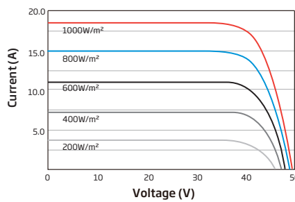
I-V CURVES OF PV MODULE (715W)
